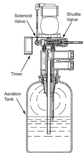
Figure 2. Air Recharge Cycle.
